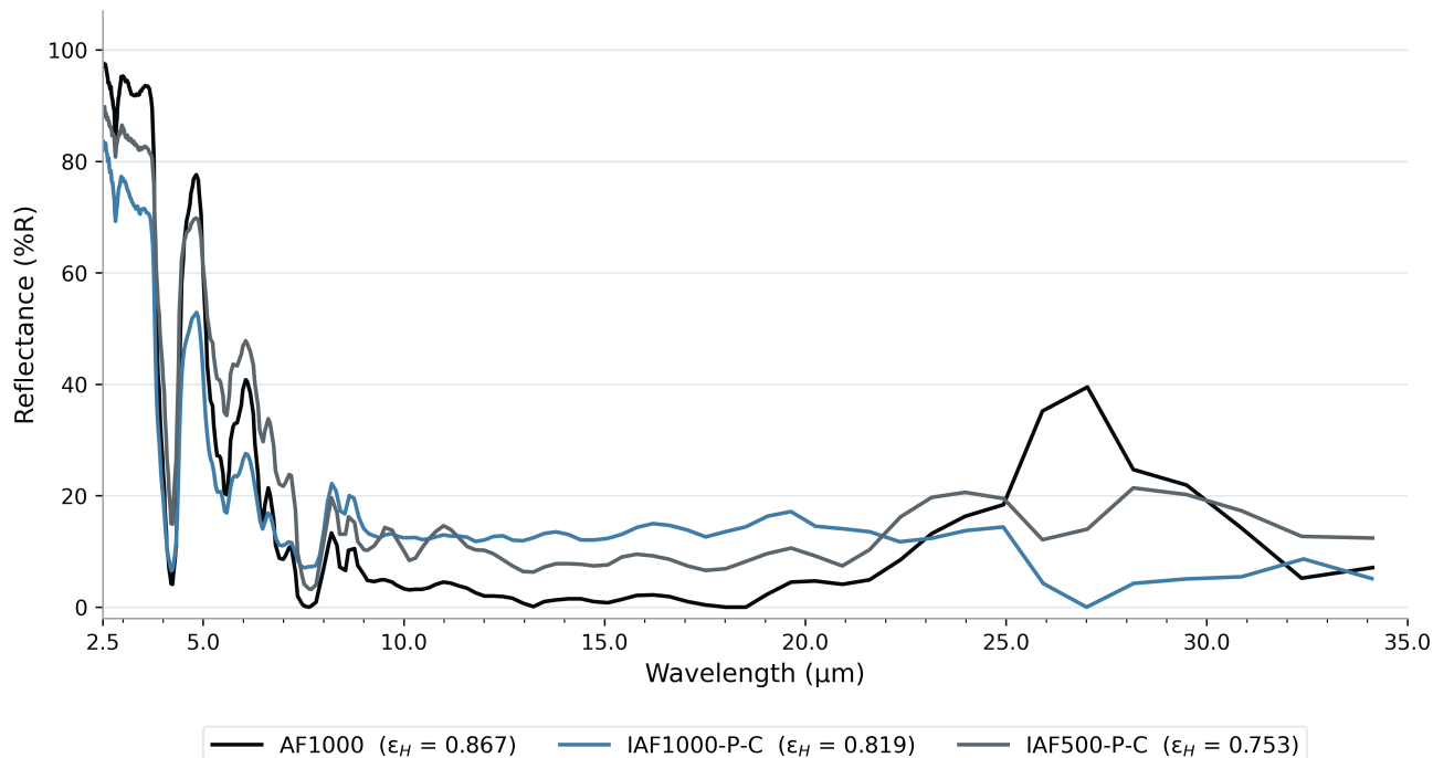
ASTM E408 Emittance Measurement
